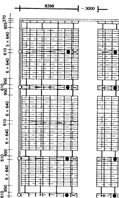
⑪ Detail of a sliding rack system for storing files
